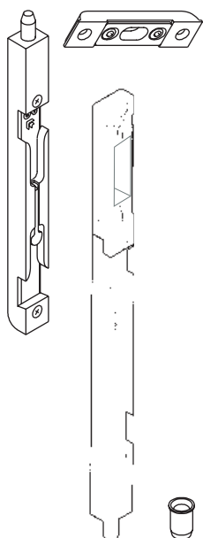
Catenaccio inf. e sup. Automatic aria 4 mm
